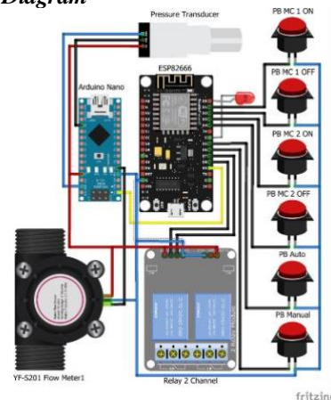
Gambar 7. Wiring Diagram
