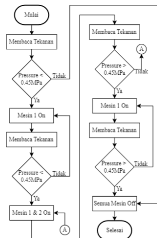
Gambar 15. Flowchart Mode Auto
