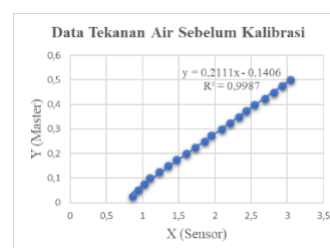
Gambar 17. Grafik Linearitas Sensor Pressure Transducer Pertama
