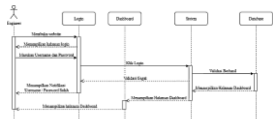
Gambar 20. Sequence Diagram Login Engineer
