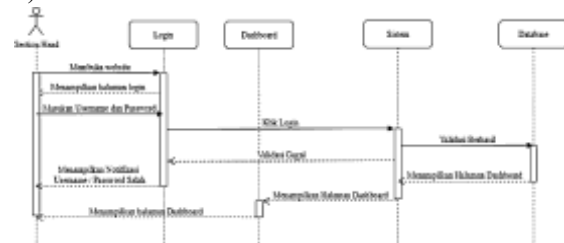
Gambar 14. Sequence Diagram Login Section Head
