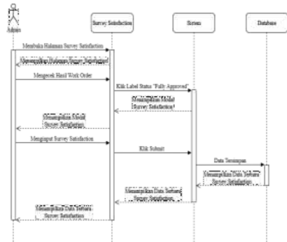
Gambar 12. Sequence Diagram Survey Satisfaction Admin
