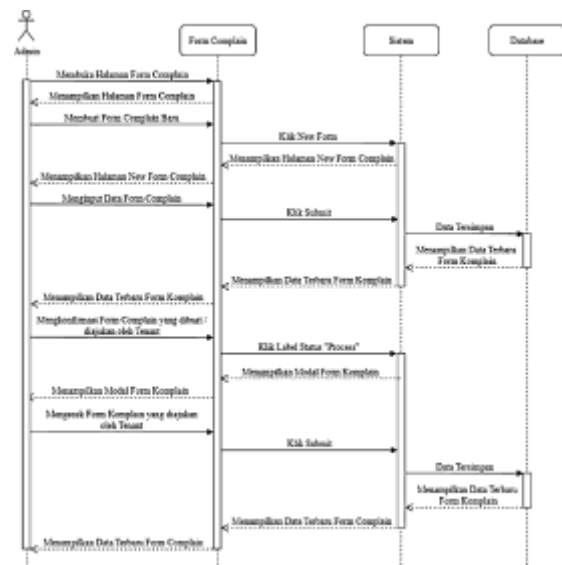
Gambar 9. Sequence Diagram Form Complain Admin
