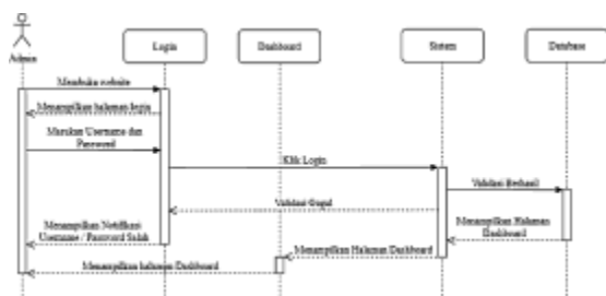
Gambar 7. Sequence Diagram Login Admin
