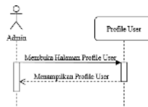
Gambar 8. Sequence Diagram Profile User Admin
