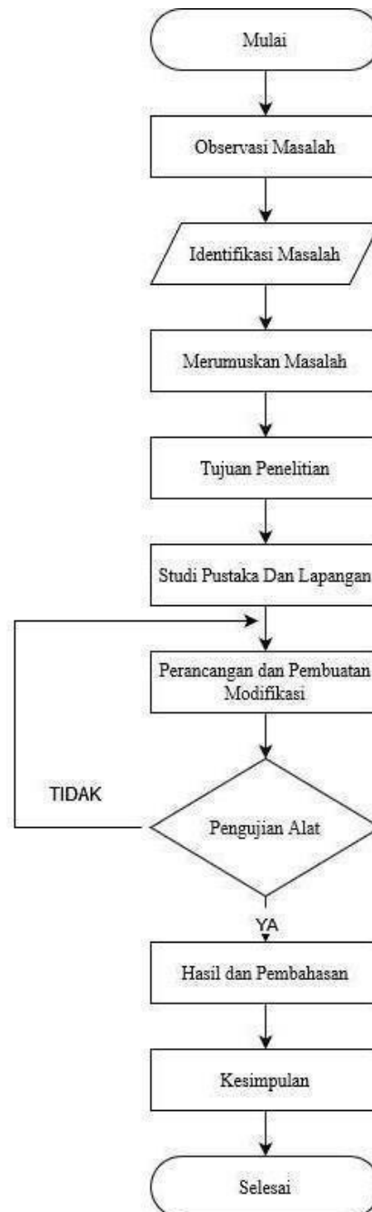
Gambar 5 Alur Penelitian
