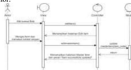
Gambar 25. Sequence Diagram Edit Master Item
