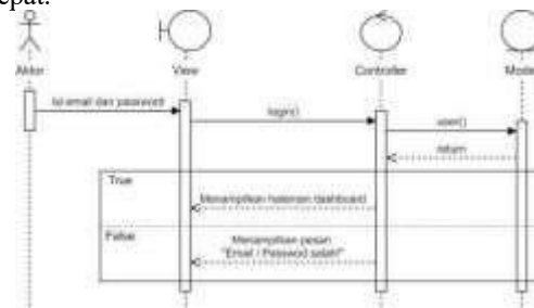
Gambar 21. Sequence Diagram Login
