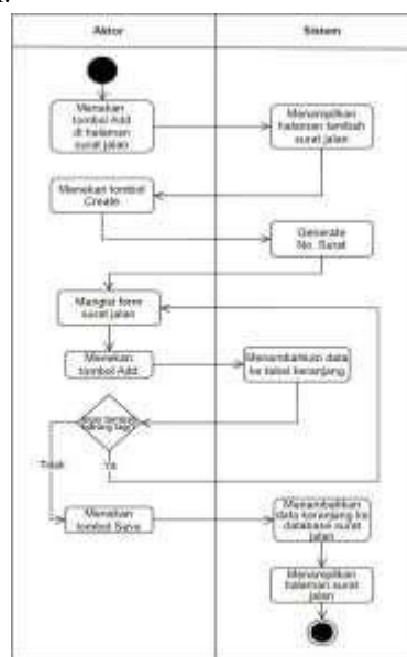
Gambar 13. Activity Diagram Add Surat Jalan
