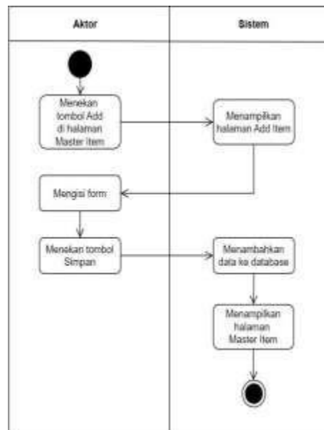
Gambar 8. Activity Diagram Add Master Item
