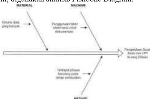
Gambar 2. . Fishbone Diagram
