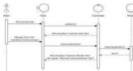
Gambar 24. Sequence Diagram Add Master Item
