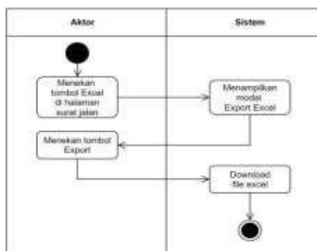
Gambar 12. Activity Diagram Export Excel Surat Jalan
