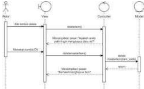
Gambar 26. Sequence Diagram Delete Master Item
