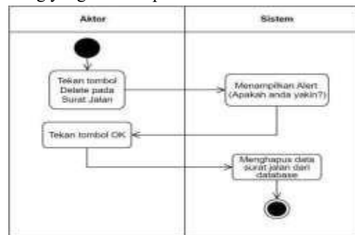
Gambar 15. Delete Surat Jalan
