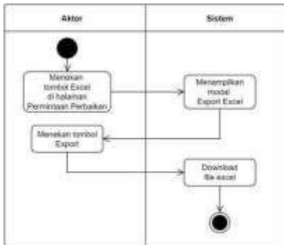
Gambar 17. Activity Diagram Export Excel LPP
