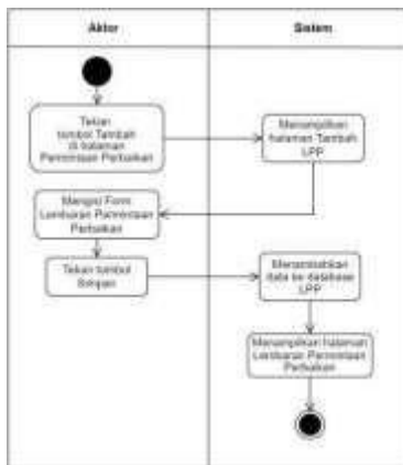
Gambar 18. Activity Diagram Tambah LPP
