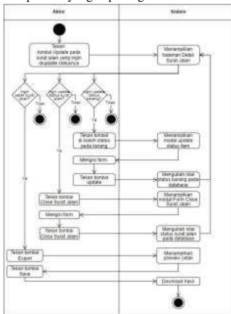
Gambar 14. Activity Diagram Update Status Surat Jalan
