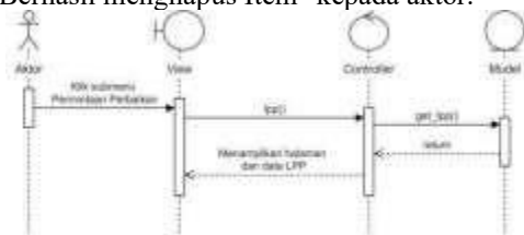
Gambar 32. Sequence Diagram LPP
