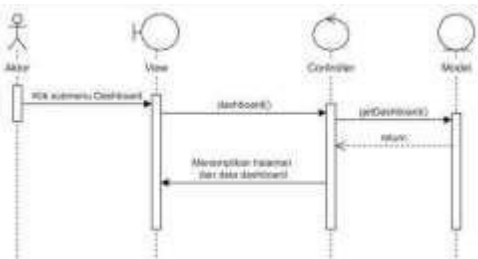
Gambar 22. Sequence Diagram Dashboard
