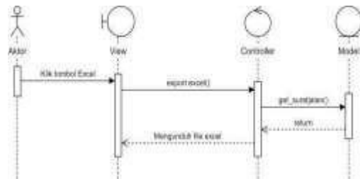
Gambar 28. Sequence Diagram Export Excel Surat Jalan
