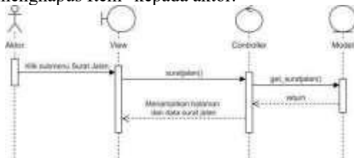
Gambar 27. Sequence Diagram Surat Jalan
