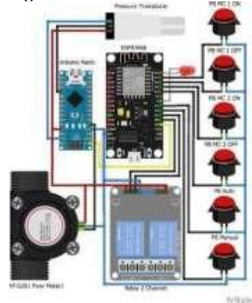
Gambar 7. Wiring Diagram
