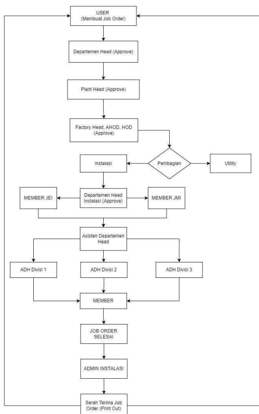
Gambar 1. Flowchart Alur Pengajuan Formulir Job Order
