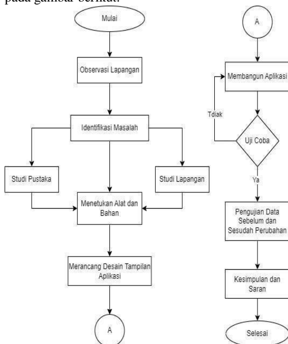
Gambar 3. Alur Penelitian
