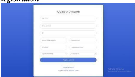
Gambar 16. Tampilan Registration
