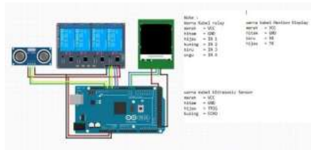
Gambar 14. Wiring Diagram Monitoring
