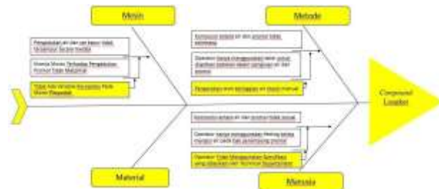
Gambar 3. Diagram Fishbone
