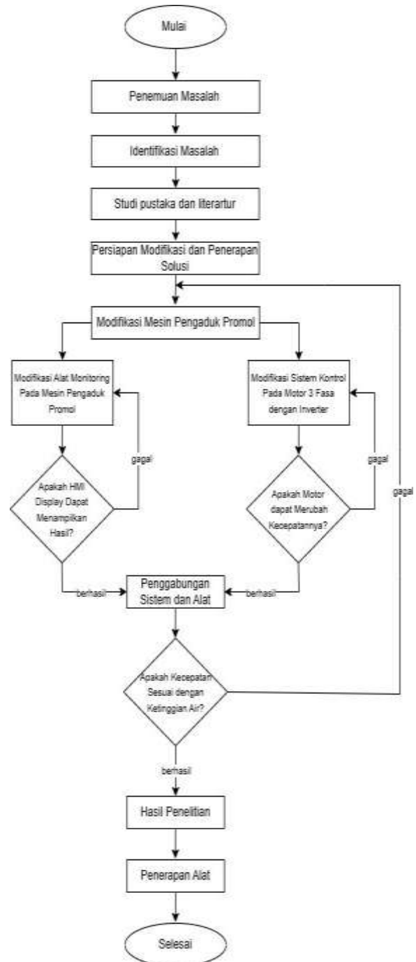
Gambar 9. Flowchart Penelitian
